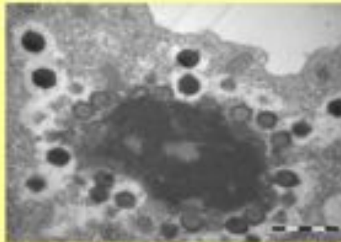
APMV particle assembling around the amoeba nucleus
