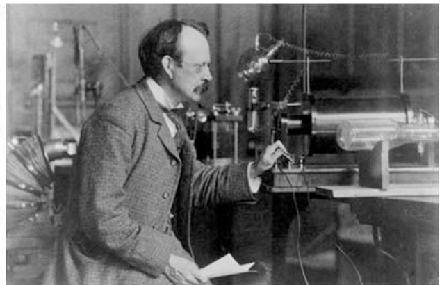
Tube cathodique (Thomson)
